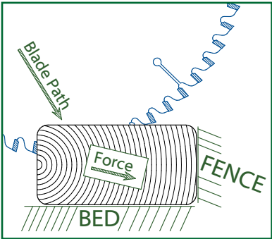
GOOD - Blade has negative hook that is forcing the material against the bed and fence of the machine.
