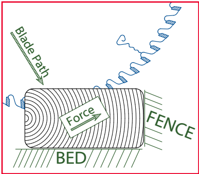
BAD - Blade has positive hook that is forcing the material away from the bed of the machine. This may result in the part being expelled.
